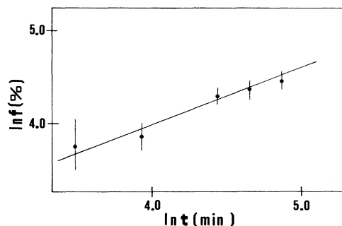
FIG. 4. Logarithmic plot showing the evolution of the fraction, f of oxidized probes as a function of the time of oxidation, for sample 4, oxidized at 550°C.
