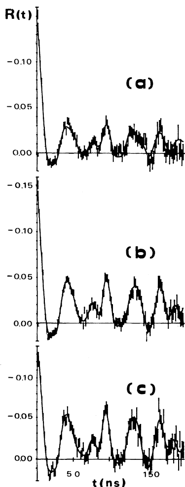
FIG. 6. TDPAC spectra of \text{In}_2\text{O}_3 measured at (a) room temperature, (b) 300°C, and (c) 550°C.
