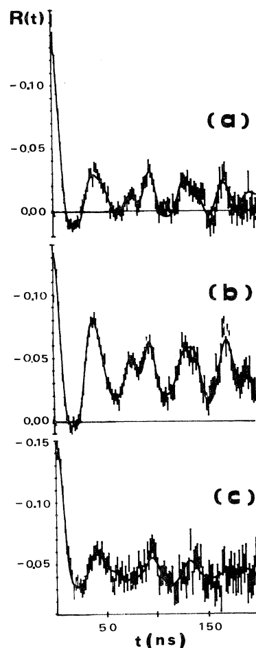
FIG. 5. TDPAC spectra at room temperature of (a) \text{In}_2\text{O}_3 , (b) \text{AgIn} , 1-at. % alloy oxidized at 1000°C, and (c) \text{AgIn} , 7-at. % \text{In} alloy oxidized at 550°C.
