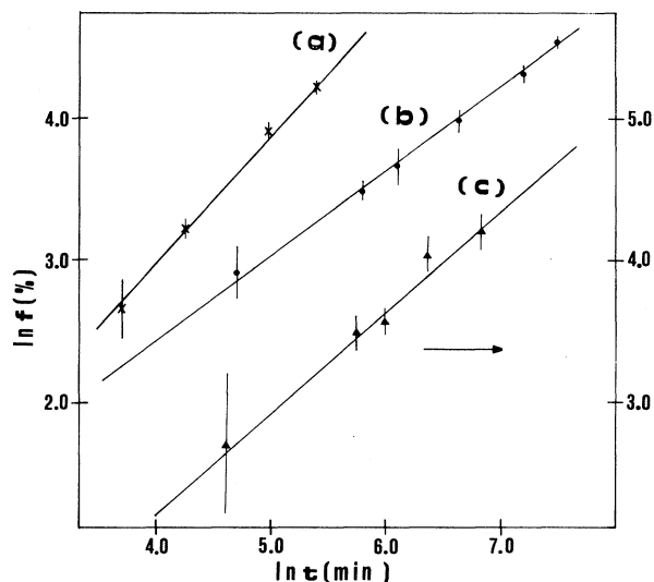
FIG. 3. Logarithmic plot showing the evolution of the fraction f of oxidized probes ( T_{\text{ox}}=300^\circ\text{C} ) as a function of the time of oxidation: (a) sample 2, (b) sample 1, and (c) sample 3.
