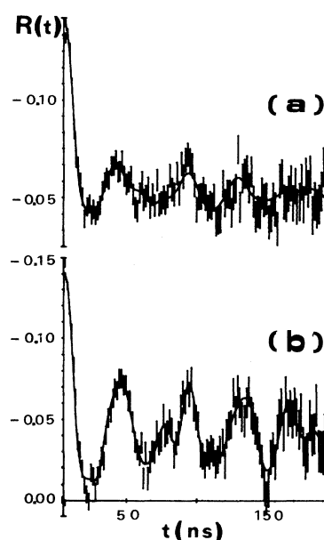
FIG. 7. TDPAC spectra of AgIn 7-at. % In alloy measured at (a) room temperature and (b) 300°C.
