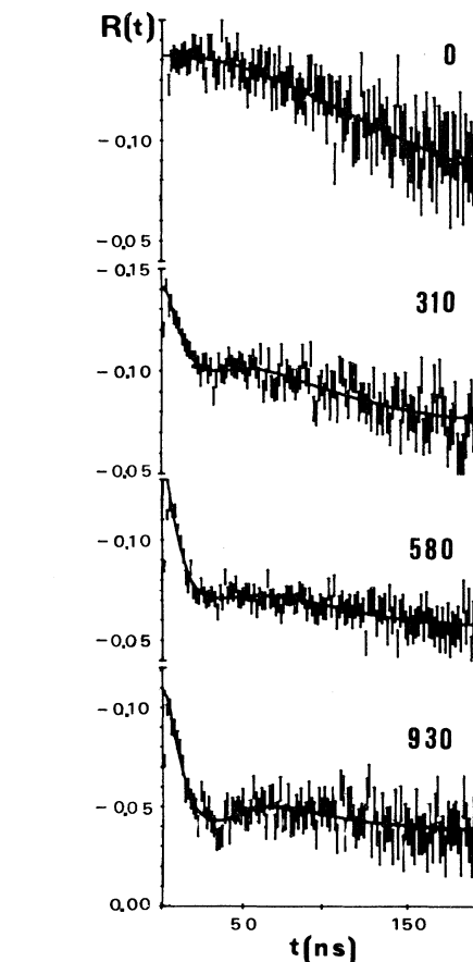
FIG. 1. TDPAC spectra after successive oxidation treatments at 300^\circ\text{C} of a 0.035-mm 1-at. % In sample preannealed at 700^\circ\text{C} for 30 min. All measurements were done at room temperature. The cumulative time of oxidation, in minutes, is indicated. Solid lines show the curves fitted to the data.
